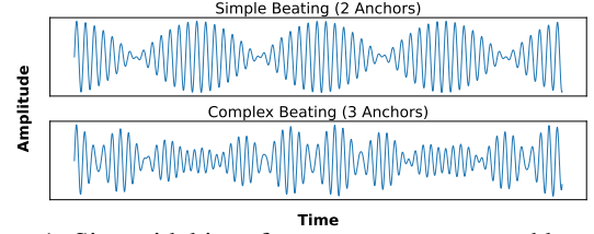
Figure 1: Sinusoidal interference patterns created by simple (2 anchors) and complex ( > 2 anchors) beating [31].
