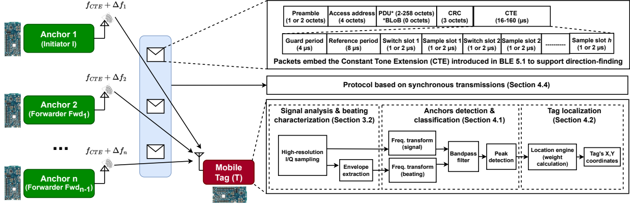
Figure 3: Overview of BLoB, a localization system that uses up to n spatially-separated single-antenna anchors synchronously transmitting packets embedding the CTE to localize single-antenna mobile tags by examining the beating characteristics across the received signal. One of the anchors acts as initiator (I) and is responsible for time-synchronizing all network operations.
