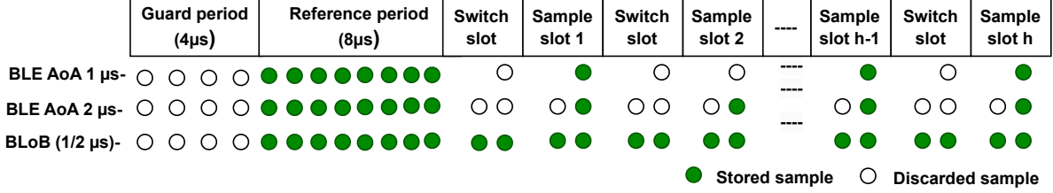
Figure 2: Overview of CTone sampling and of the stored I/Q samples at the receiver. Classical systems (e.g., AoA-based [26]) store h = 74 or h = 37 I/Q samples when using 1\mu\text{s} - or 2\mu\text{s} -long antenna-switching and sampling slots. In contrast, BLoB uses a single antenna and leverages the antenna-switching slot for extra I/Q sampling, which results in up to h = 148 collected samples.
