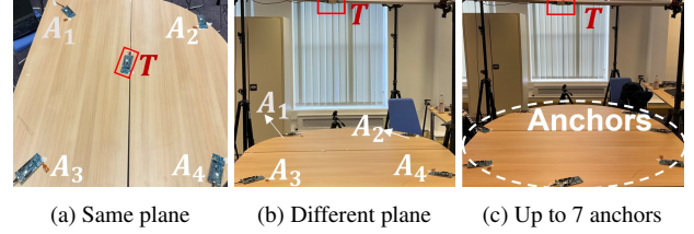
Figure 7: Experimental setup used in § 5.1.
