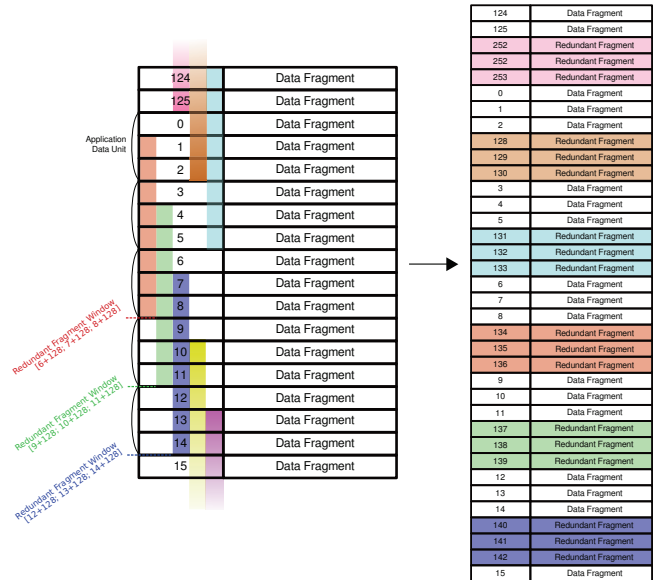
Figure 1: Fragment computation window and numbering, w = 8 and each ADU contains 3 fragments.
