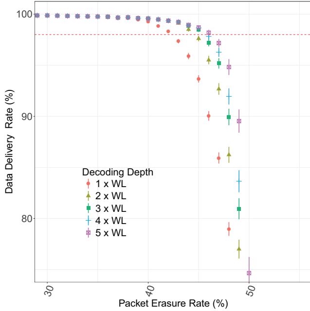
Figure 7: Simulated DDR as a function of PER with LoRaFFEC (128;0.6;DD) for various DD.
