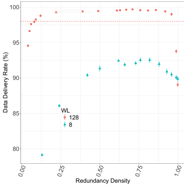
Figure 6: Simulated DDR as a function of RD with LoRaFFEC (128;RD;2) and LoRaFFEC (8;RD;2) over a 40% erasure channel.
