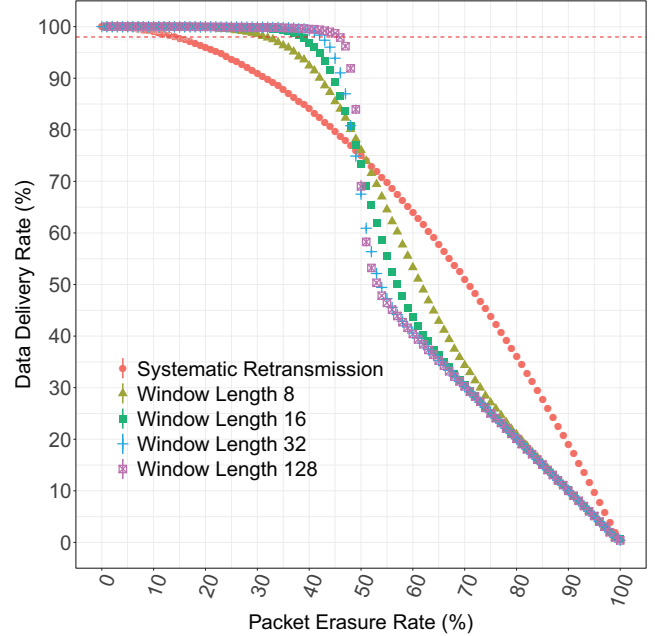
Figure 5: Simulated DDR as a function of PER with LoRaFFEC (w; 0.6; 5) .
