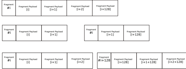
Figure 4: Aggregation of data and redundancy fragments into LoRaWAN TM frames.
