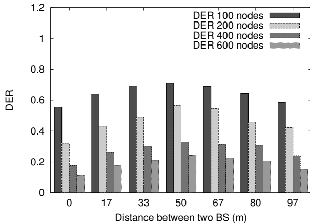
Figure 5. Impact of distance between two base stations on DER for different number of nodes.
