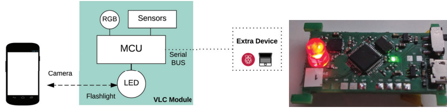
Figure 2. On the left, the demonstration block diagram. On the right, our demo board
