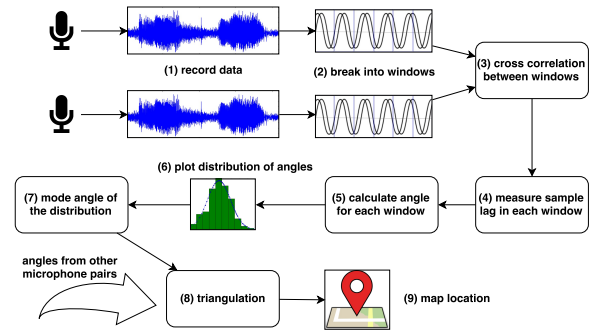
Figure 2: Process of calculating the location of an elephant. A pair of infrasonic detectors capture elephant sounds.
