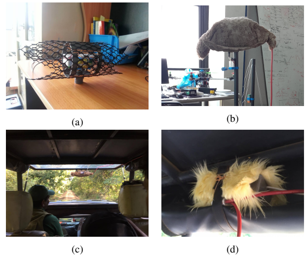
Figure 1: (a) The microphone together with the pre-amp circuitry is placed inside a sealed plastic box and then put inside the wire-frame with shock mounting. (b) Wire-frame covered with a soft material to cancel wind noise. In (c) and (d), two microphones are mounted in the front and back of a vehicle for field experiments.
