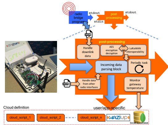
Figure 4. Modular and versatile low-cost gateway
