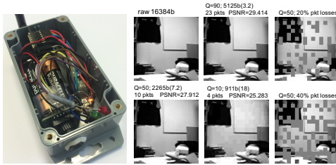
Figure 2. Long-range image sensor device
