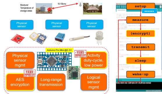
Figure 1. Generic IoT platform
