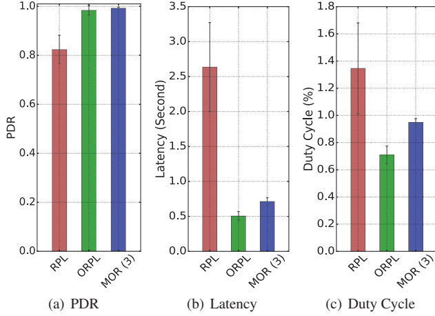
Figure 4: Effectiveness of opportunistic routing. In interference-free scenarios, ORPL performs slightly better than MOR in terms of latency and duty cycle, since it operates over a single channel, leading to less overhead than in MOR. In terms of PDR, MOR achieves similar performance to ORPL. ORPL and MOR outperform RPL on all three metrics.
